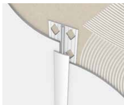
Two-part joining section
